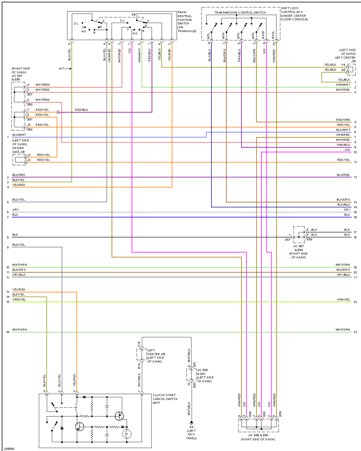
Fig. 18: 4.0L, Engine Performance Circuit (5 of 6)
