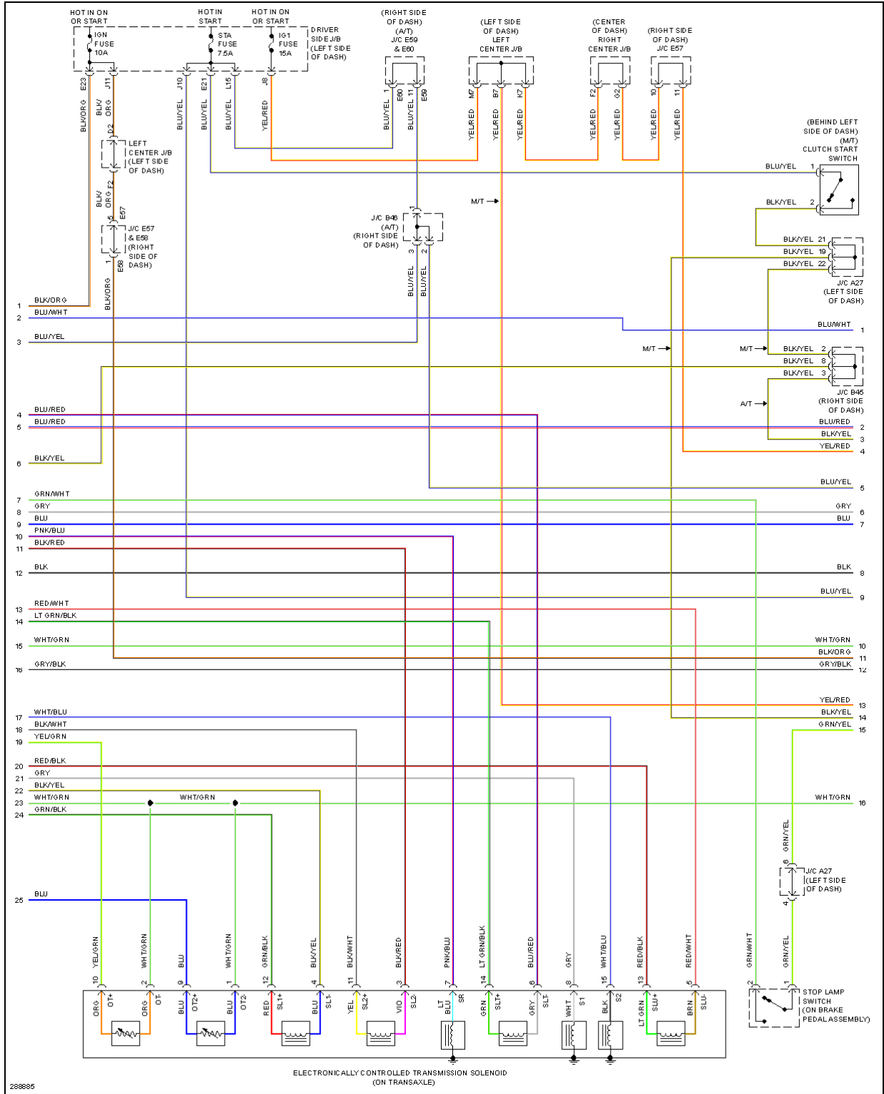
Fig. 17: 4.0L, Engine Performance Circuit (4 of 6)
