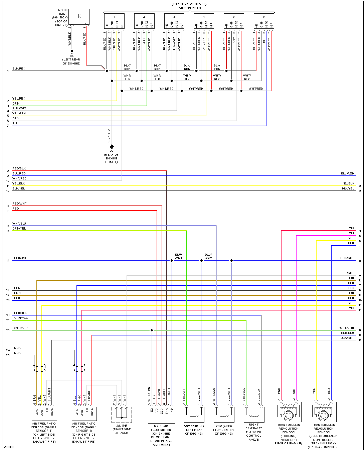
Fig. 15: 4.0L, Engine Performance Circuit (2 of 6)
