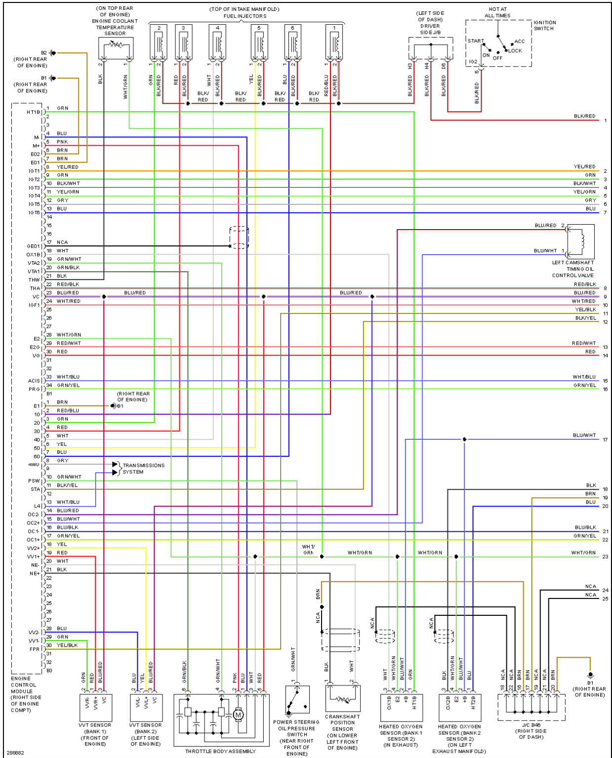
Fig. 14: 4.0L, Engine Performance Circuit (1 of 6)
