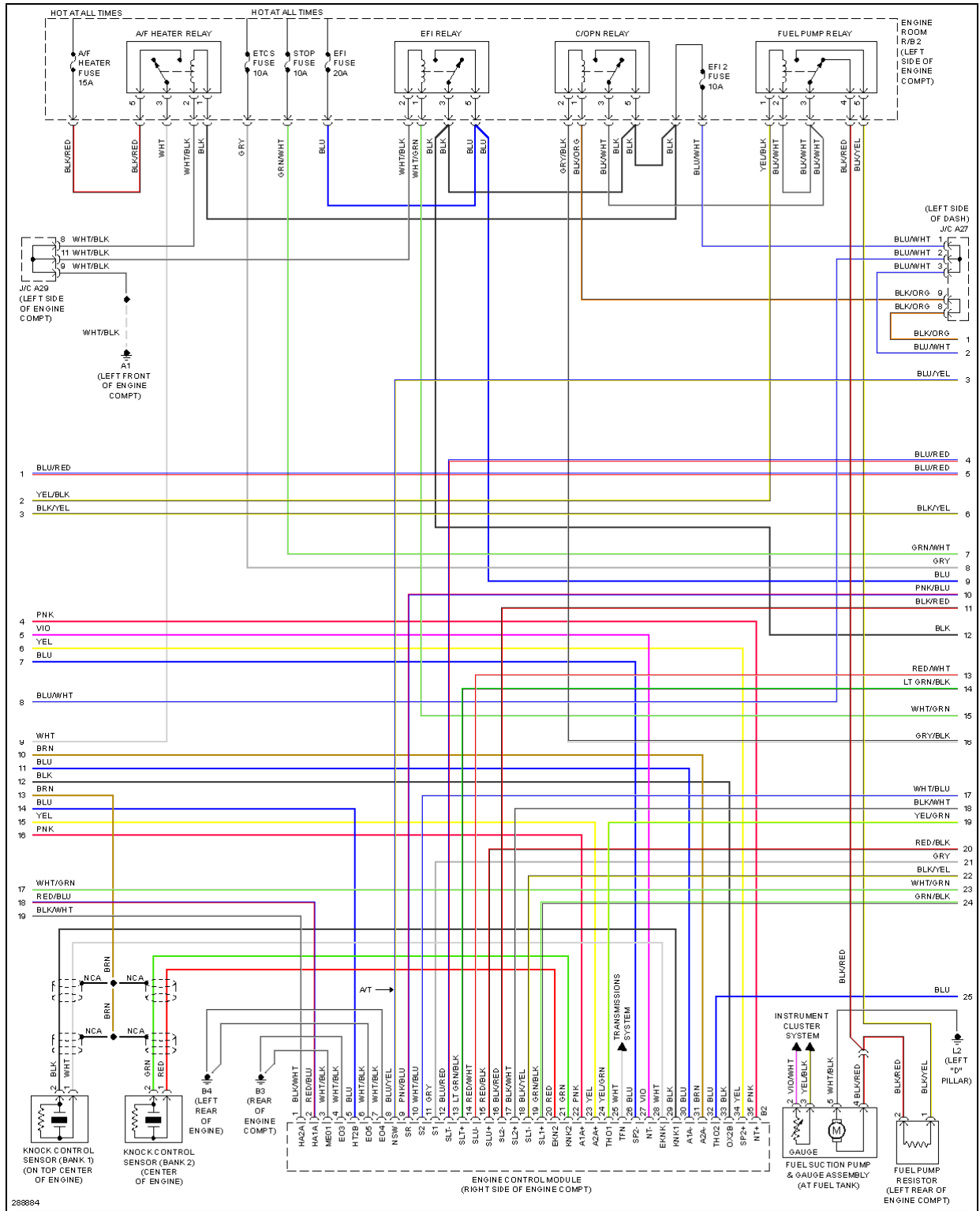
Fig. 16: 4.0L, Engine Performance Circuit (3 of 6)
