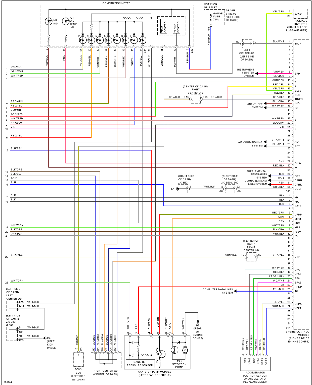
Fig. 19: 4.0L, Engine Performance Circuit (6 of 6)
